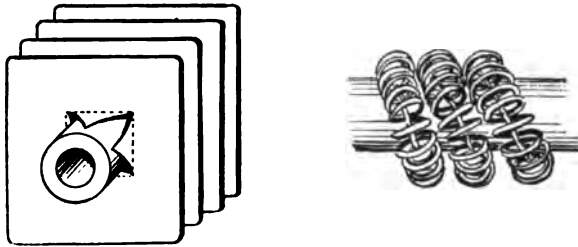
FIG. 294.—Details of Two Descriptions of Water Cooling Radiators. In the first, the pipe is surrounded by metal fins, let on as indicated; in the second, it is surrounded with coils of helical wire.
